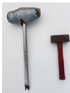
Massettes
